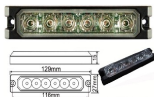
Code3 High power XT6
