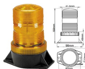
LED Vehicle Flashing Beacon 219
